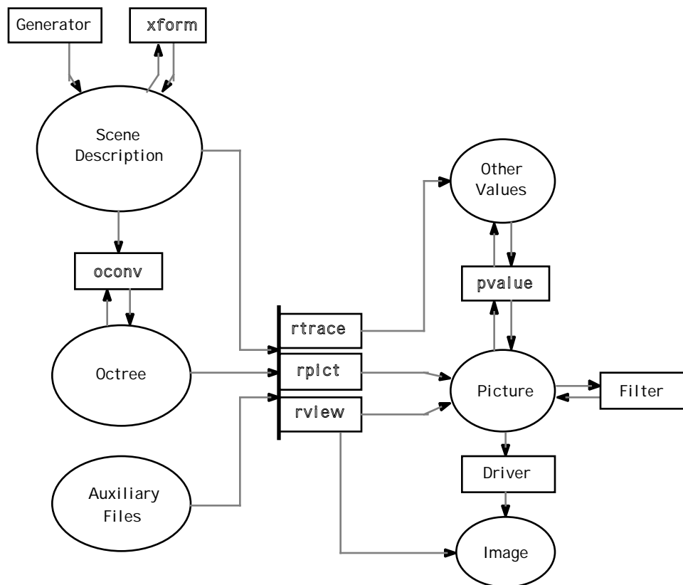
Figure 1. Programs and data flow in Radiance .
